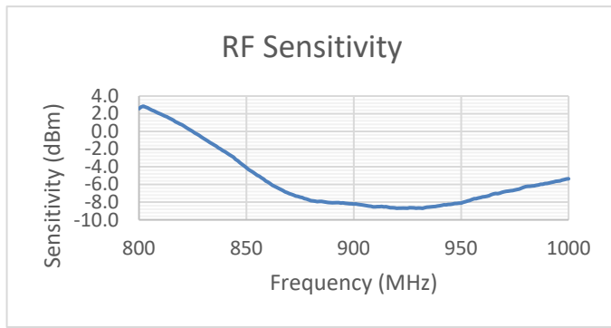
Figure 2 RF Sensitivity and Read Range of AZN5200-AFR
