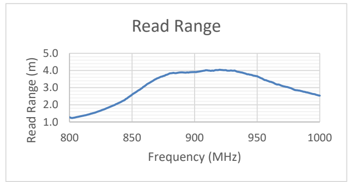
Figure 2 RF Sensitivity and Read Range of AZN5200-AFR
