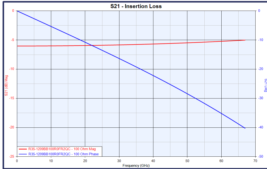
12 x 09 100 Ω Insertion Loss
